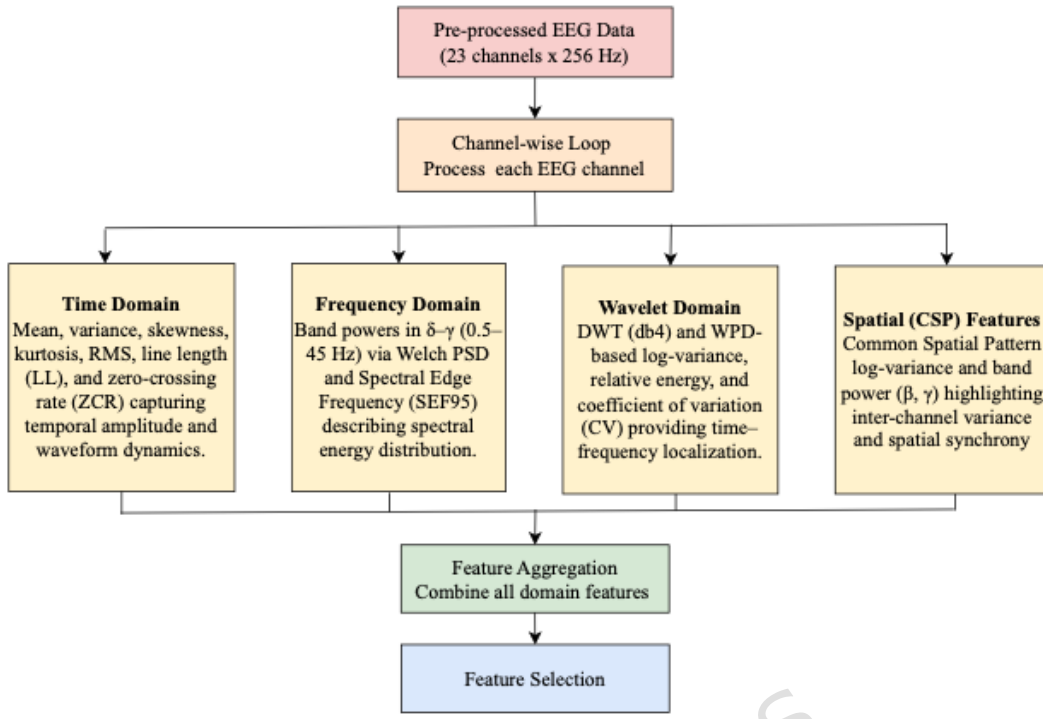
Figure 3: Our multi-domain feature extraction process, showing parallel analysis of time, frequency, wavelet, and spatial domains, followed by feature selection and classification.
