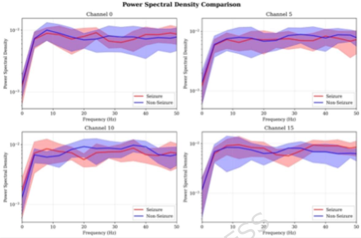
Figure 9: Power Spectral Density comparisons showing characteristic spectral elevation during seizure activity, particularly in beta and gamma bands.
