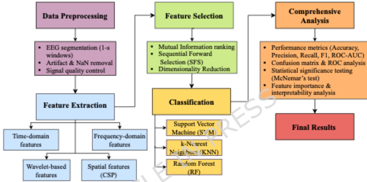
Figure 1: Our complete EEG seizure detection process from raw data to classification outcome.
